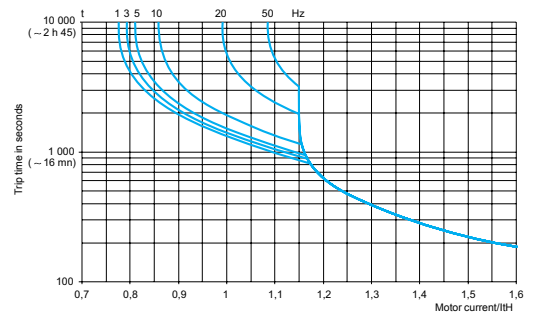
Motor thermal protection curves
